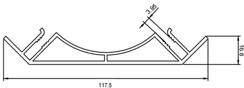
LM-04 阴角型材
